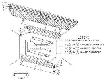
FIG. 1. Storage-ring interaction region and detector system for 556-MeV electron scattering experiment.
