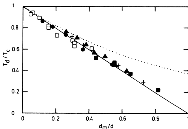
FIG. 2. Universal plot: T_d/T_c vs d_m/d . The full line is Eq. (8) and the dotted line is Cooper's law, Eq. (23). The experimental points are as follows Nb (Ref. 4) = □ ( d_m = 36 Å) and ■ ( d_m = 22 Å); Pb (Ref. 5) = ● ( d_m = 8 Å) and ▲ ( d_m = 20 Å); and Bi (Ref. 5) = + ( d_m = 12 Å).
