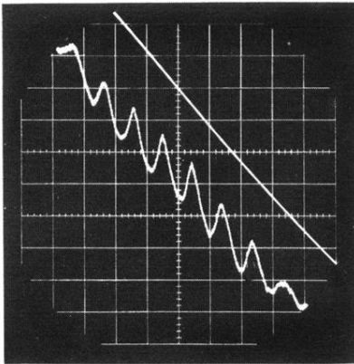
FIG. 4. Lower trace: variation of the resistance of tin cylinder with magnetic field after differentiation which reduces the quadratic background to a linear background. Upper trace: magnetic field sweep.
