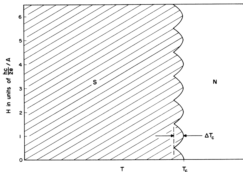
FIG. 1. Phase diagram for a thin cylindrical superconductor in an axial magnetic field. The scalloped edge of the superconducting phase results from the periodicity in the free energy of the bound pairs, in the magnetic flux through the cylinder.
