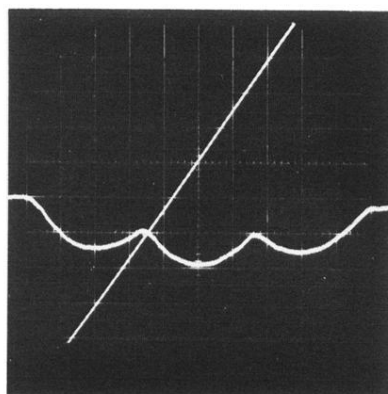
FIG. 3. Enlarged view of parabolic variation of the resistance of tin cylinder for pairs in quantum states -1 , 0 , and +1 . Straight line is magnetic field variation with zero field at the center of the picture.
