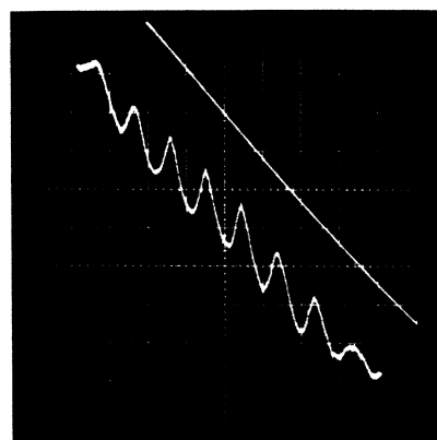
FIG. 4. Lower trace: variation of the resistance of tin cylinder with magnetic field after differentiation which reduces the quadratic background to a linear background. Upper trace: magnetic field sweep.
